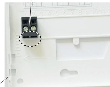
Base plate: connection, power supply wires
