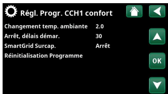
Menu «Avancé/Réglages/Circ Chauffage/Circ Chauffage 1/Programme/Confort».
